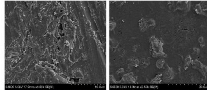
Figure 9. SEM micrographs of abraded X80 steel immersed in 1 M HCl (left) and in 1 M HCl containing 10 \times 10^{-5} M FLU (right).
